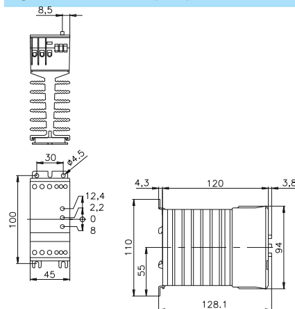
fig. 2. Dimensions (mm)
