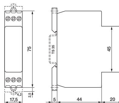
fig. 2. Dimension (mm)
