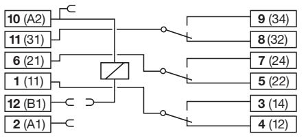
Connection diagram S3-MB0
