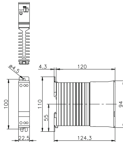
fig. 2. Dimensions (mm)
