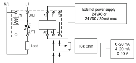
11-12: Thermostat
