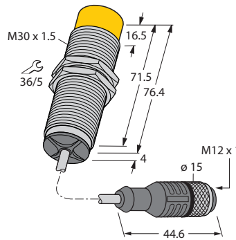
Fig. 2: Primary side NICP-M30-8P8-0,3-RSC12T
