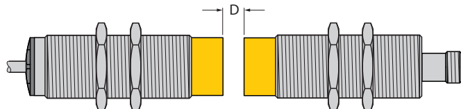
Fig. 11: Distance between primary side (right) and secondary side (left)
