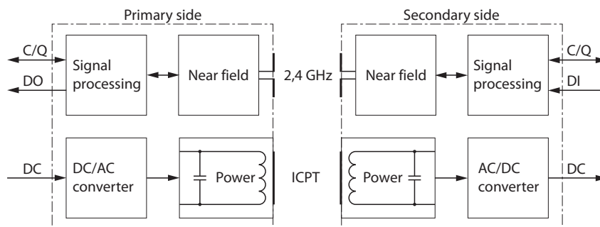
Fig. 4: Block diagram
