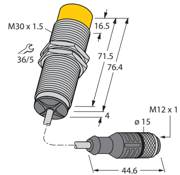
Fig. 3: Secondary side NICS-M30-IOL2P8-0,3-RKC4.4T
