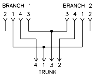
Wiring Diagram
